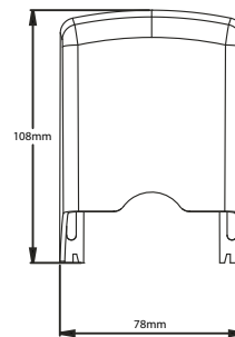
Front view of waterproof cover
